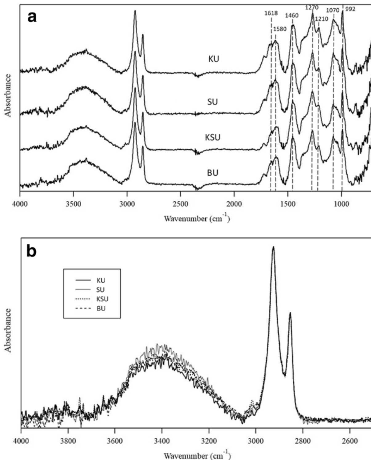
FTIR spectra of the each urushi film in the range of 4000–650 \text{cm}^{-1} (a) and magnified figure of broad band between 3600 and 3200 \text{cm}^{-1} (b)
